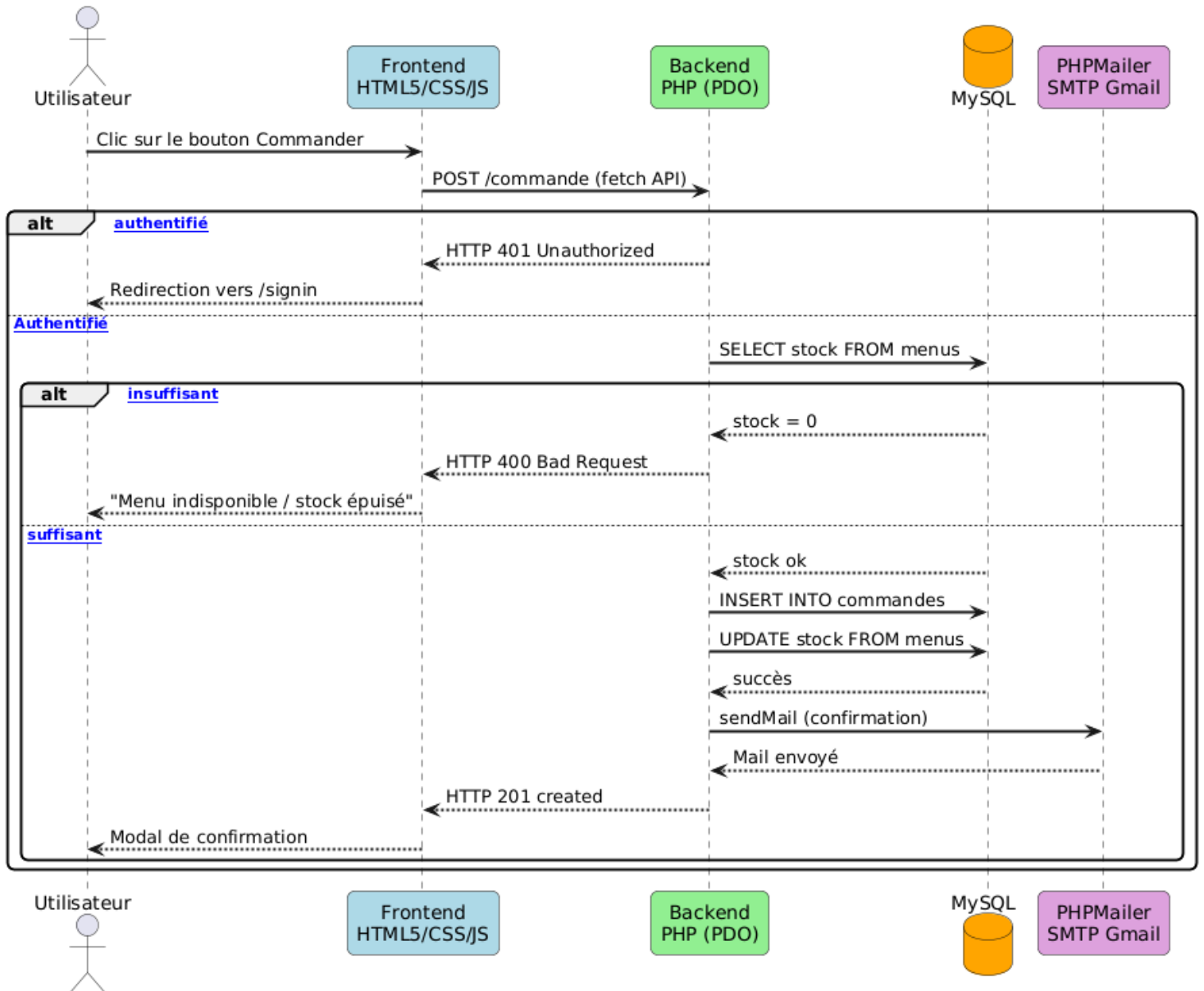
Diagramme_sequence_commande_menu
